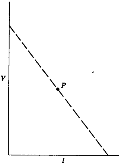
FIG. 8-6.— (V, I) -characteristic of a line-type pulser.
